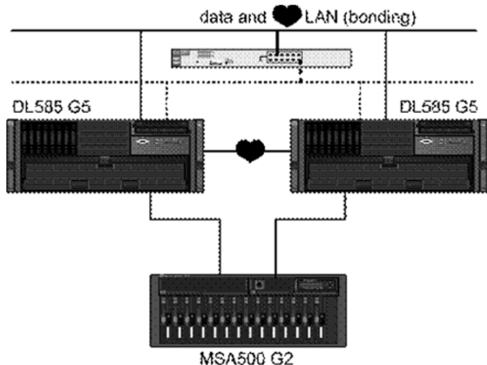
Figure 1: HP's recommended cluster configuration for SCSI in a switch attach configuration.
